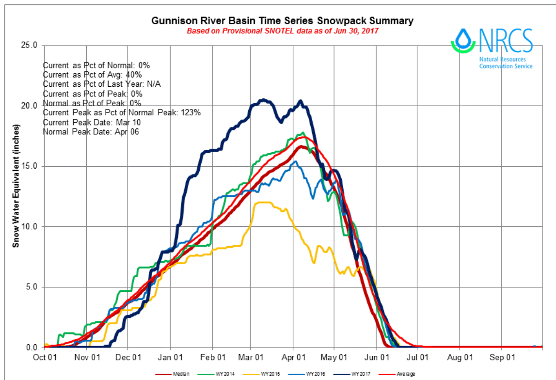
Figure 3: Comparison of this season's water year (navy blue line), relative to previous seasons and the 30 year average for the Gunnison River Basin. The snowpack was below average until mid-December, but then it skyrocketed in January to nearly 200% of average at many SNOTELS.
