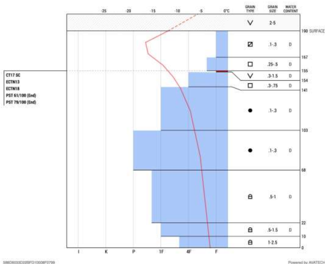
Figure 24: 1/28/17. Snodgrass study plot showing a deep and fairly consistent snow profile with the exception of the January 19 surface hoar layer in the upper snowpack.
