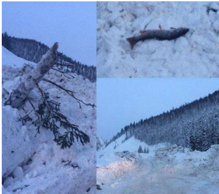
Figure 18: Destructive debris crossed Taylor Canyon highway and river on 1/12/17, burying the popular fishing site below Taylor Reservoir.
