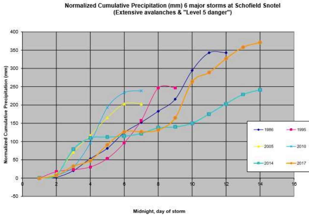
Figure 17: Cumulative snow water equivalent from the January 2017 cycle surpassed all previous major storms ever recorded at Schofield Pass SNOTEL since its installation in 1986 (although technically, this cycle was two separate storms).
