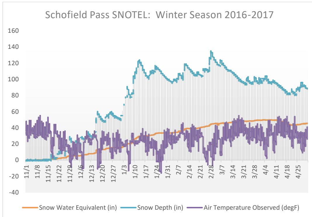
Figure 2: Air temperature, snow water equivalent, and snow depth measurements from Schofield Pass SNOTEL, at 10,700 ft. Schofield Pass is in the orographically favored “snow belt” of the Elk Mountains.
