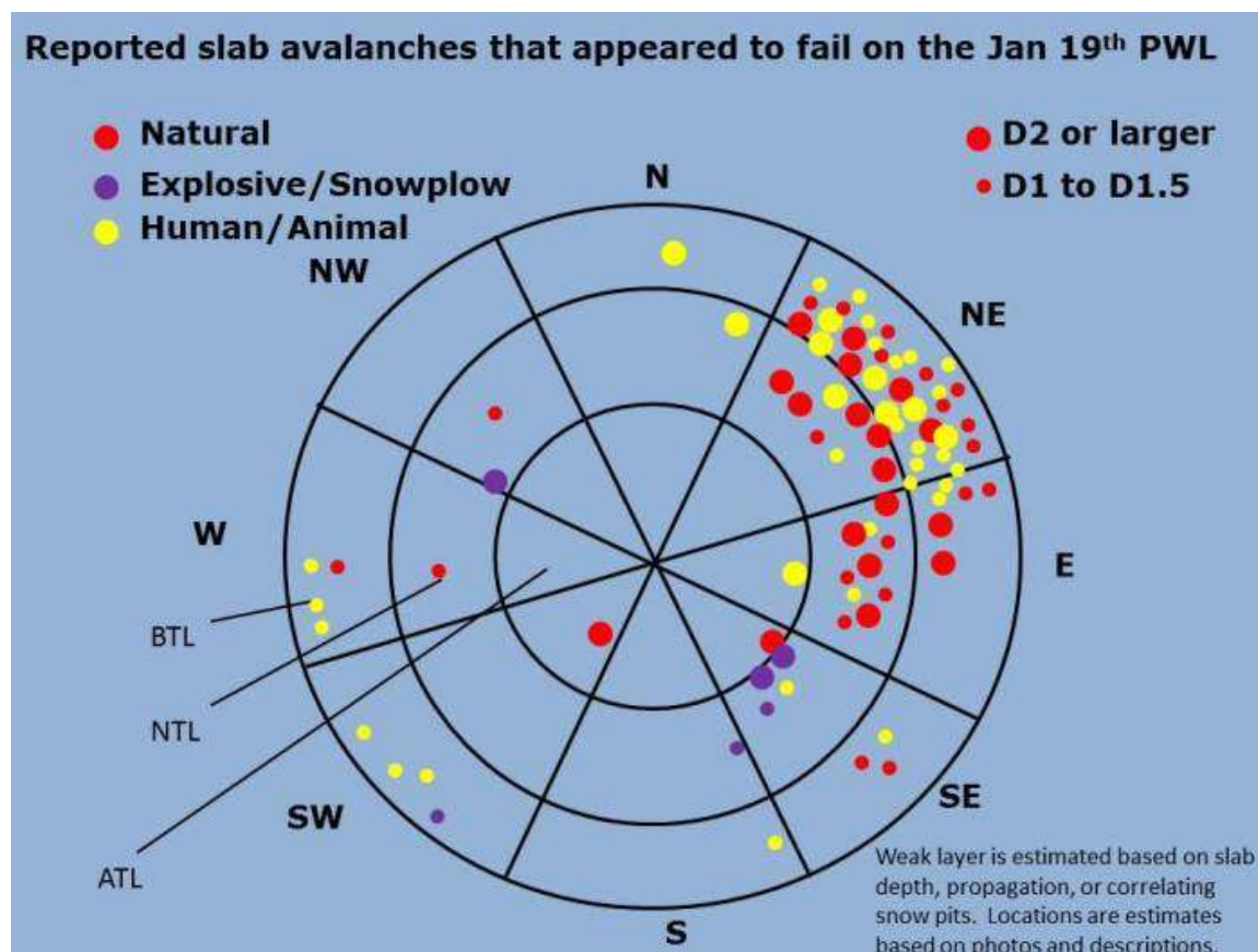
Figure 23: January avalanche activity on the January 19th surface hoar layer. This layer remained active well into February.
